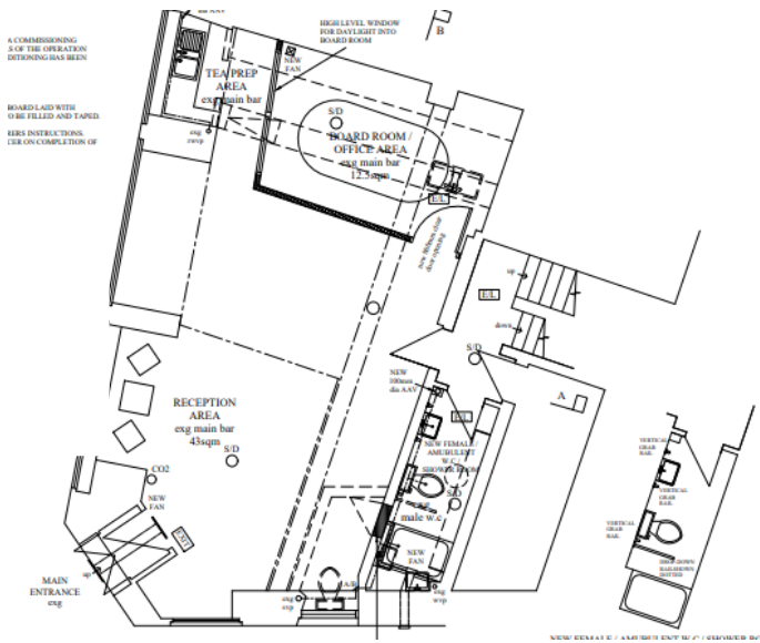
Ground Floor 1
